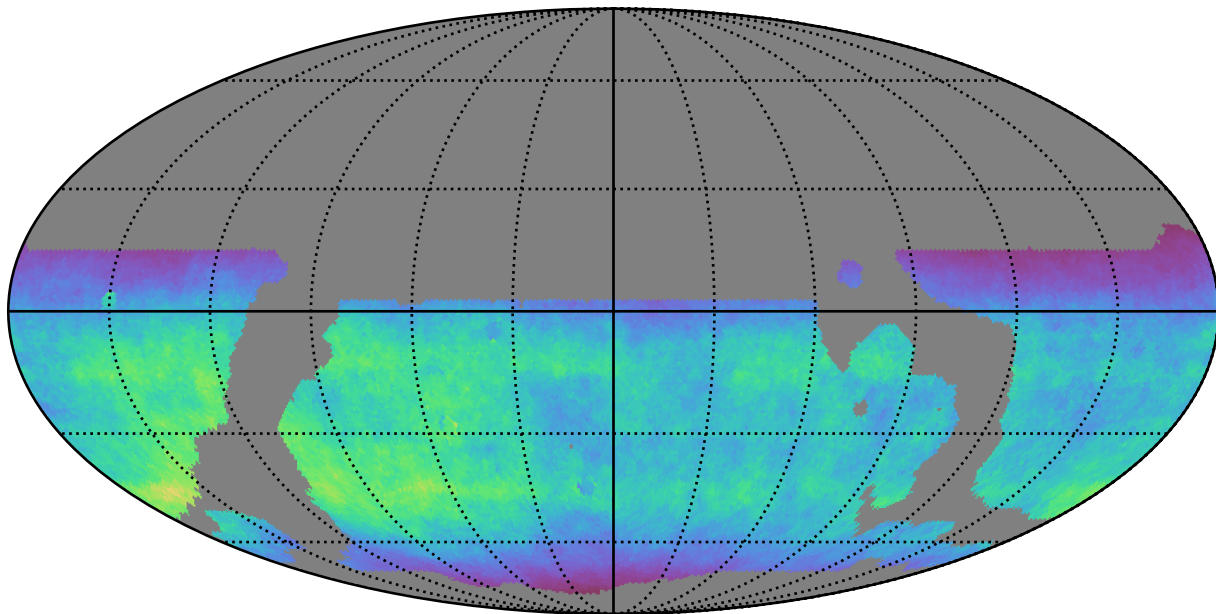
weather_cloudso10v3.4_10yrs WFD y band: Normalized Teff
