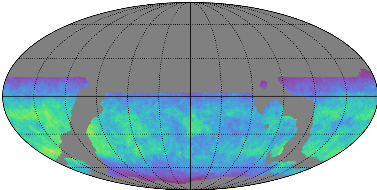
weather_cloudso10v3.4_10yrs WFD u band: Normalized Teff
