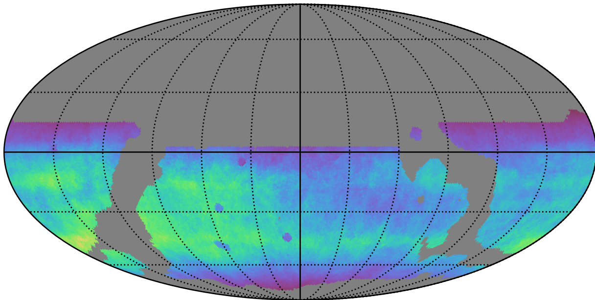
weather_cloudso10v3.4_10yrs WFD r band: Normalized Teff
