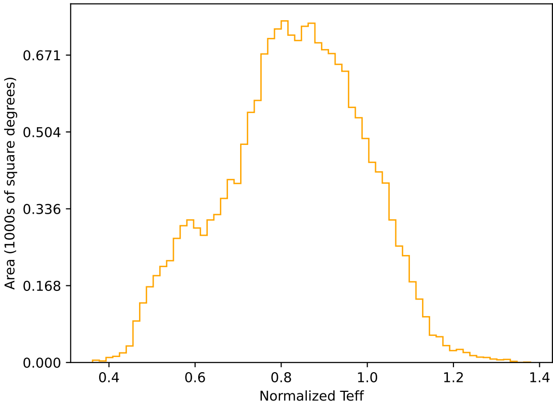
weather_cloudso10v3.4_10yrs WFD r band: Normalized Teff
