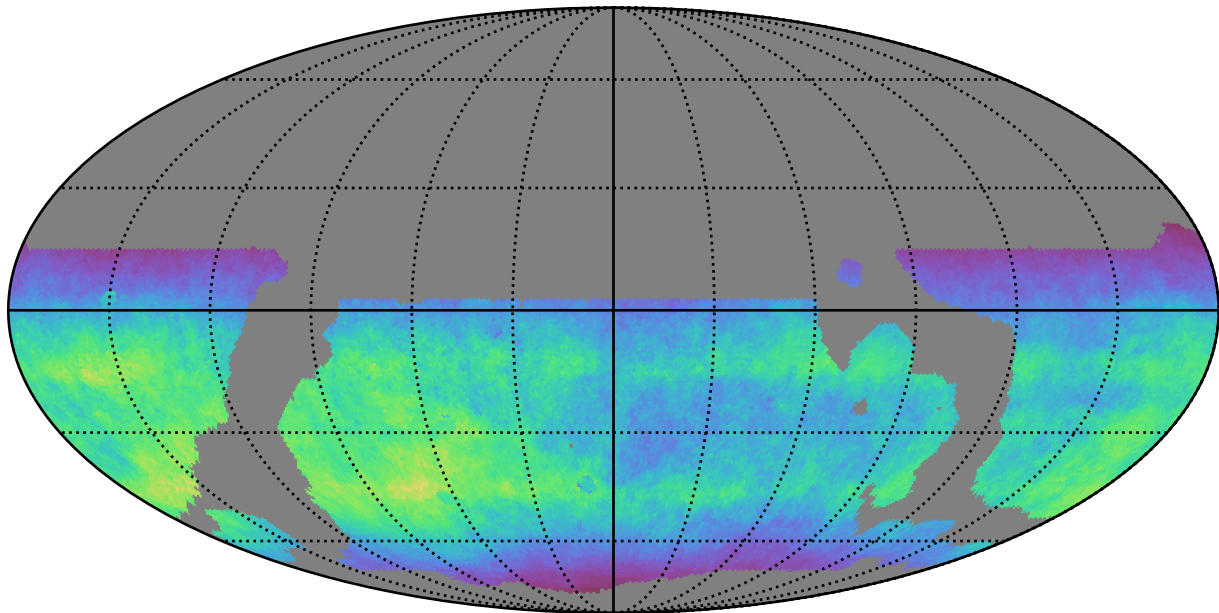
weather_cloudso10v3.4_10yrs WFD i band: Normalized Teff
