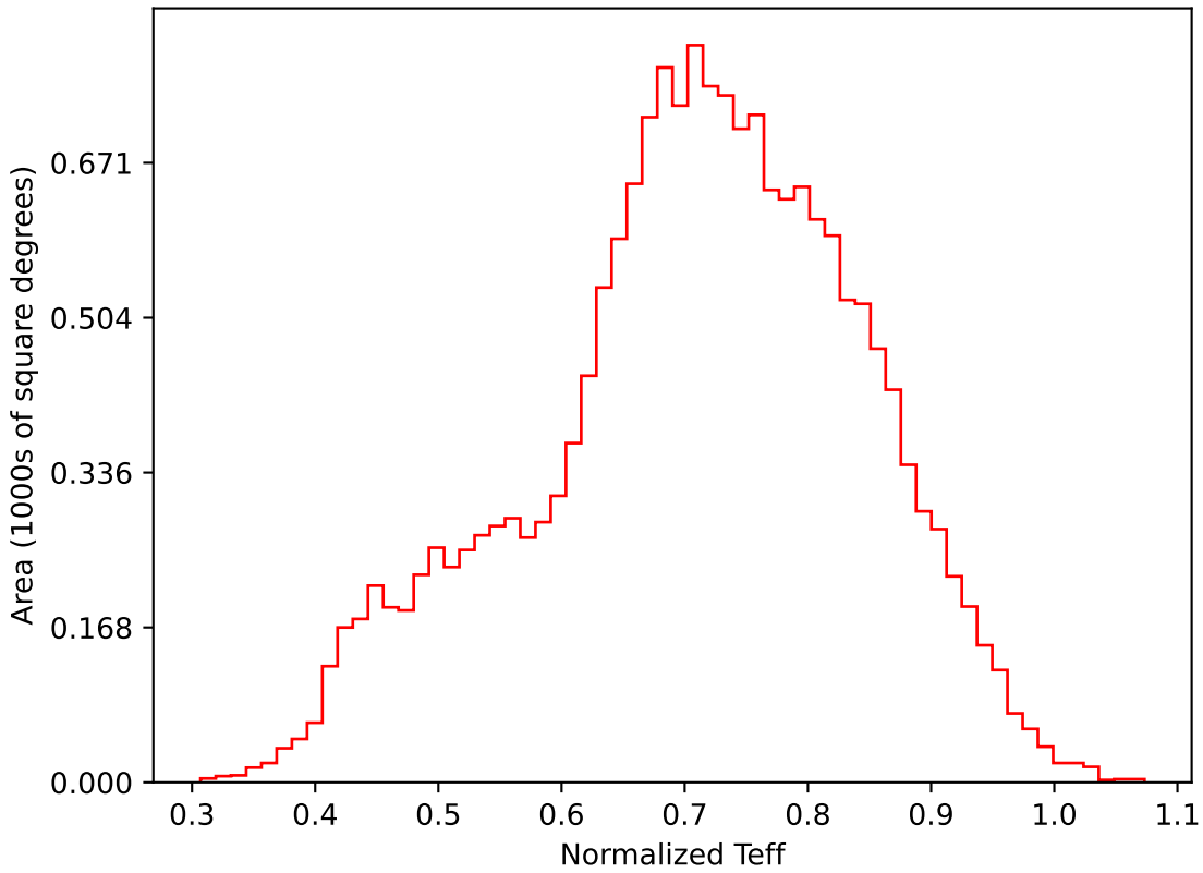
weather_cloudso10v3.4_10yrs WFD i band: Normalized Teff
