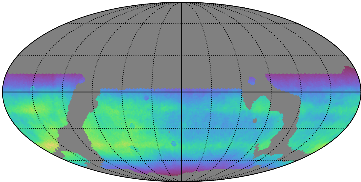
weather_cloudso10v3.4_10yrs WFD all bands: Normalized Teff
