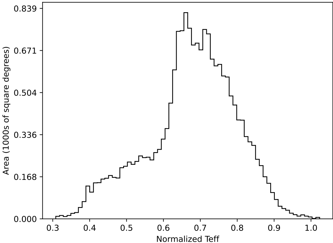
weather_cloudso10v3.4_10yrs WFD all bands: Normalized Teff
