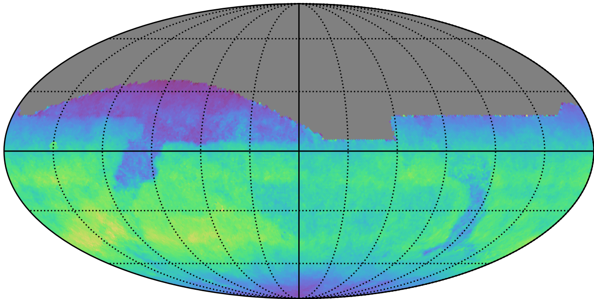
weather_cloudso10v3.4_10yrs All sky z band: Normalized Teff
