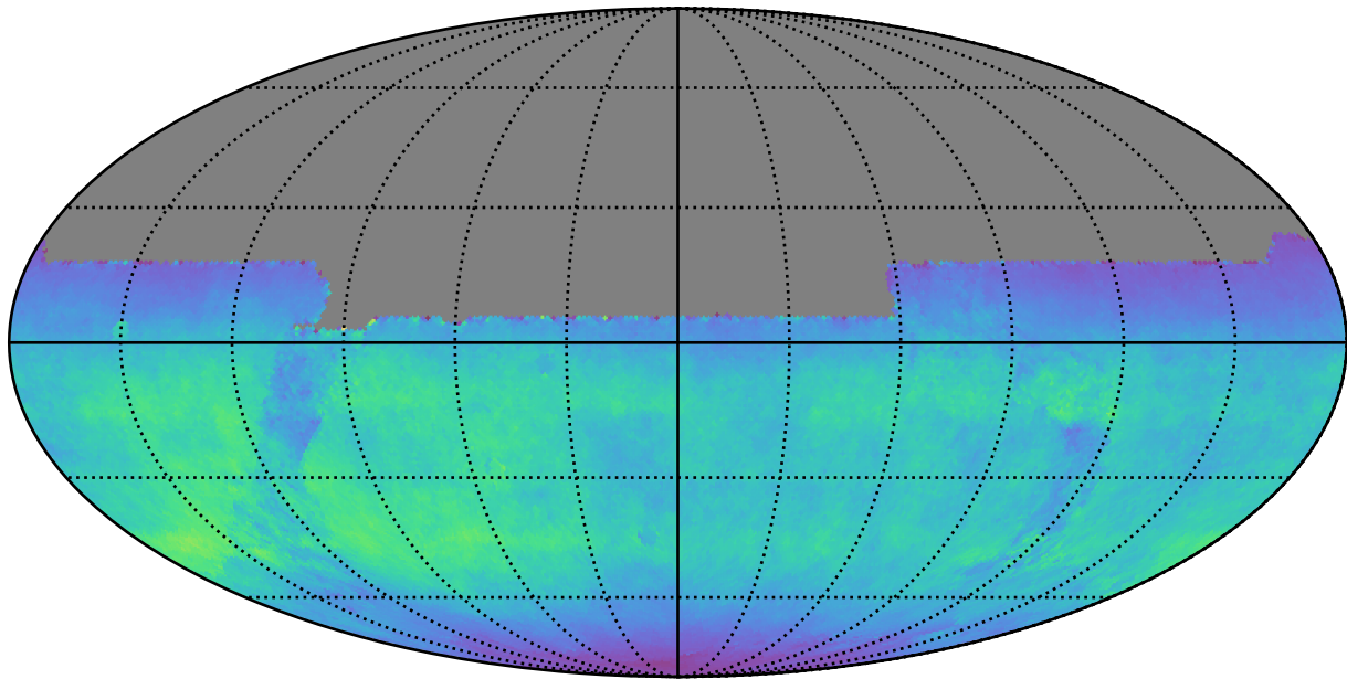
weather_cloudso10v3.4_10yrs All sky y band: Normalized Teff
