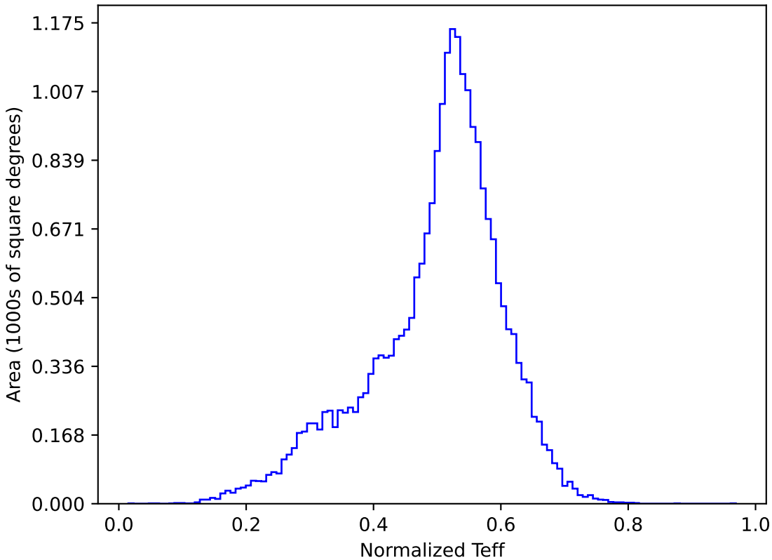
weather_cloudso10v3.4_10yrs All sky y band: Normalized Teff
