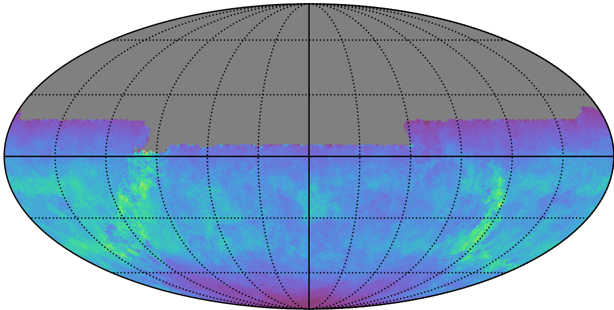
weather_cloudso10v3.4_10yrs All sky u band: Normalized Teff
