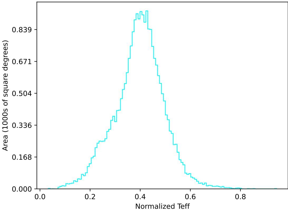
weather_cloudso10v3.4_10yrs All sky u band: Normalized Teff
