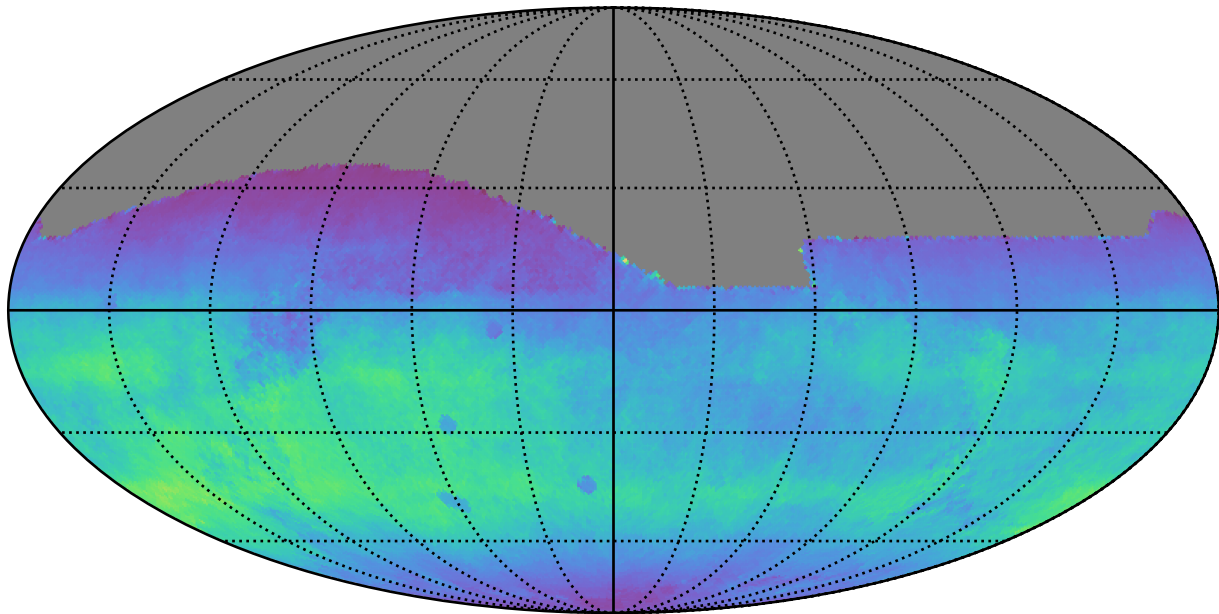
weather_cloudso10v3.4_10yrs All sky r band: Normalized Teff
