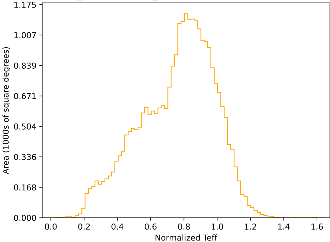
weather_cloudso10v3.4_10yrs All sky r band: Normalized Teff
