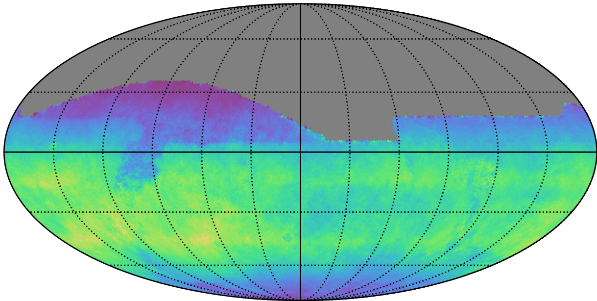
weather_cloudso10v3.4_10yrs All sky i band: Normalized Teff
