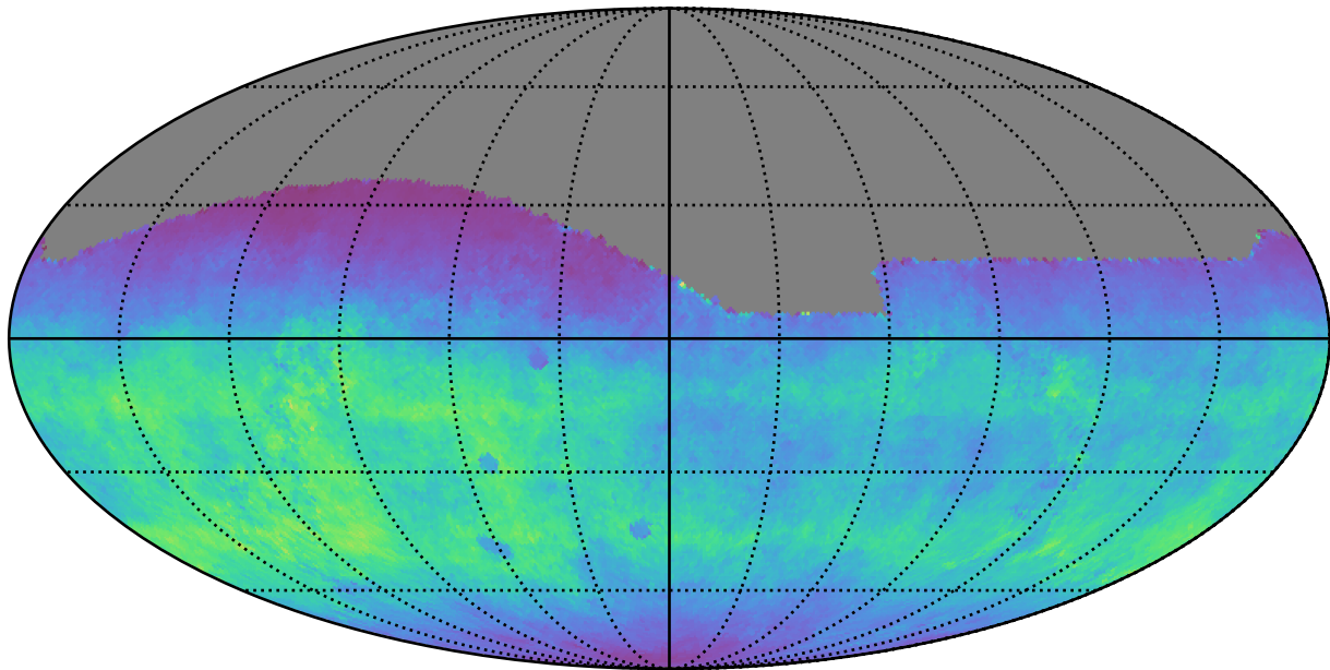
weather_cloudso10v3.4_10yrs All sky g band: Normalized Teff
