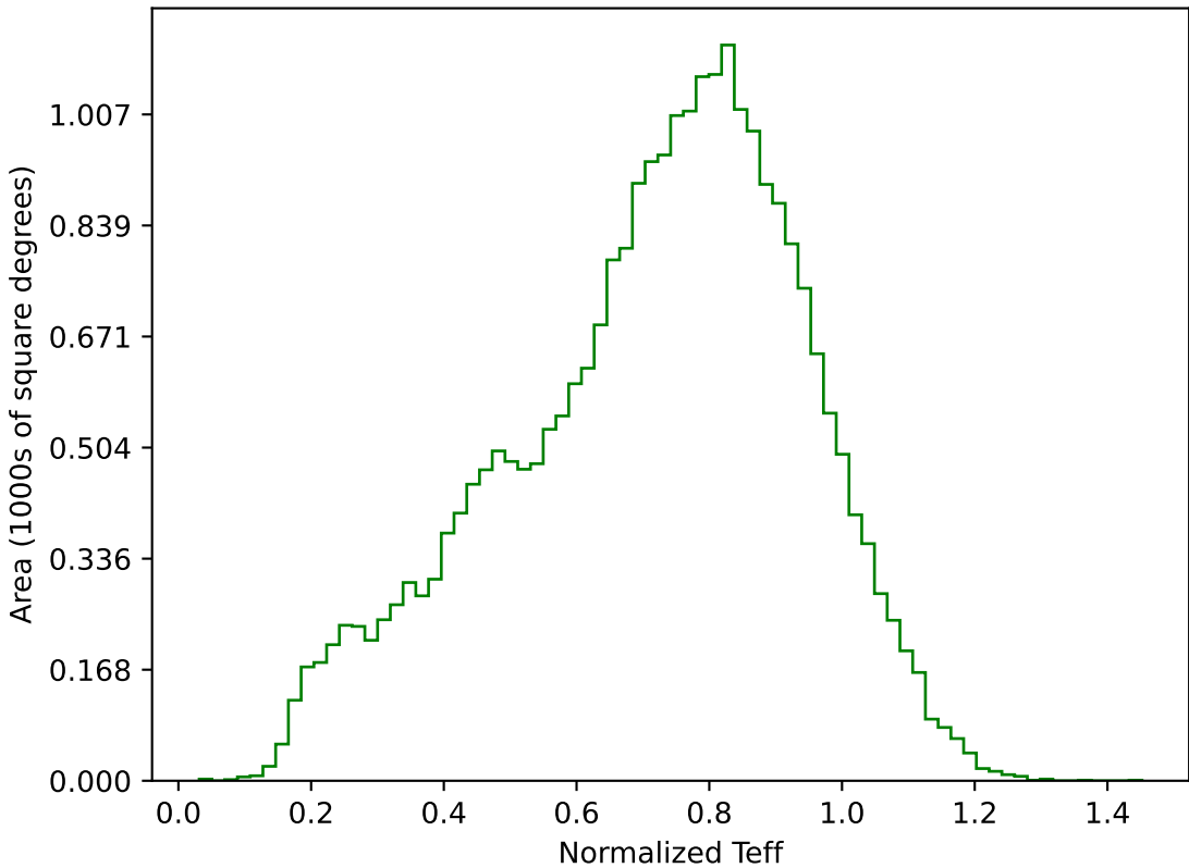
weather_cloudso10v3.4_10yrs All sky g band: Normalized Teff
