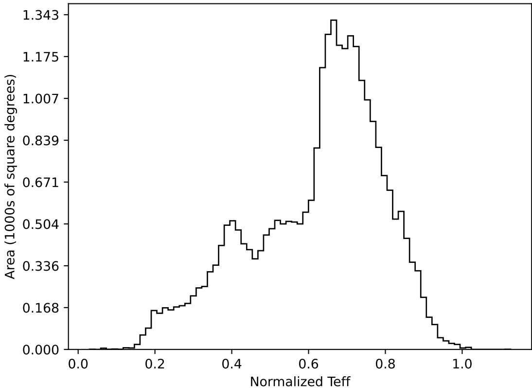
weather_cloudso10v3.4_10yrs All sky all bands: Normalized Teff
