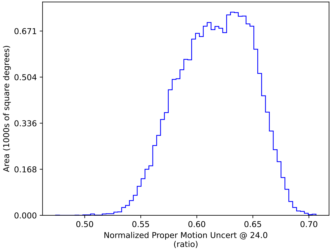
weather_cloudso10v3.4_10yrs WFD: Normalized Proper Motion Uncert @ 24.0
