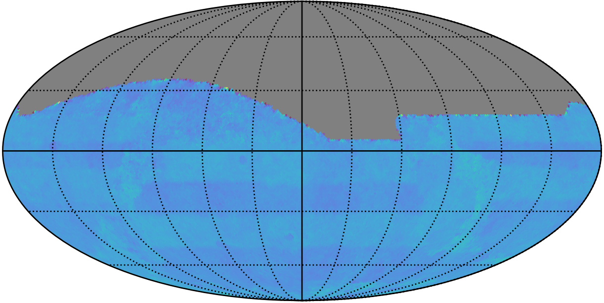
weather_cloudso10v3.4_10yrs All sky: Normalized Proper Motion Uncert @ 24.0
