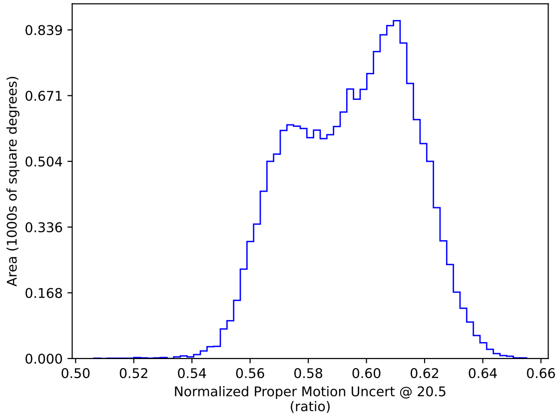
weather_cloudso10v3.4_10yrs WFD: Normalized Proper Motion Uncert @ 20.5
