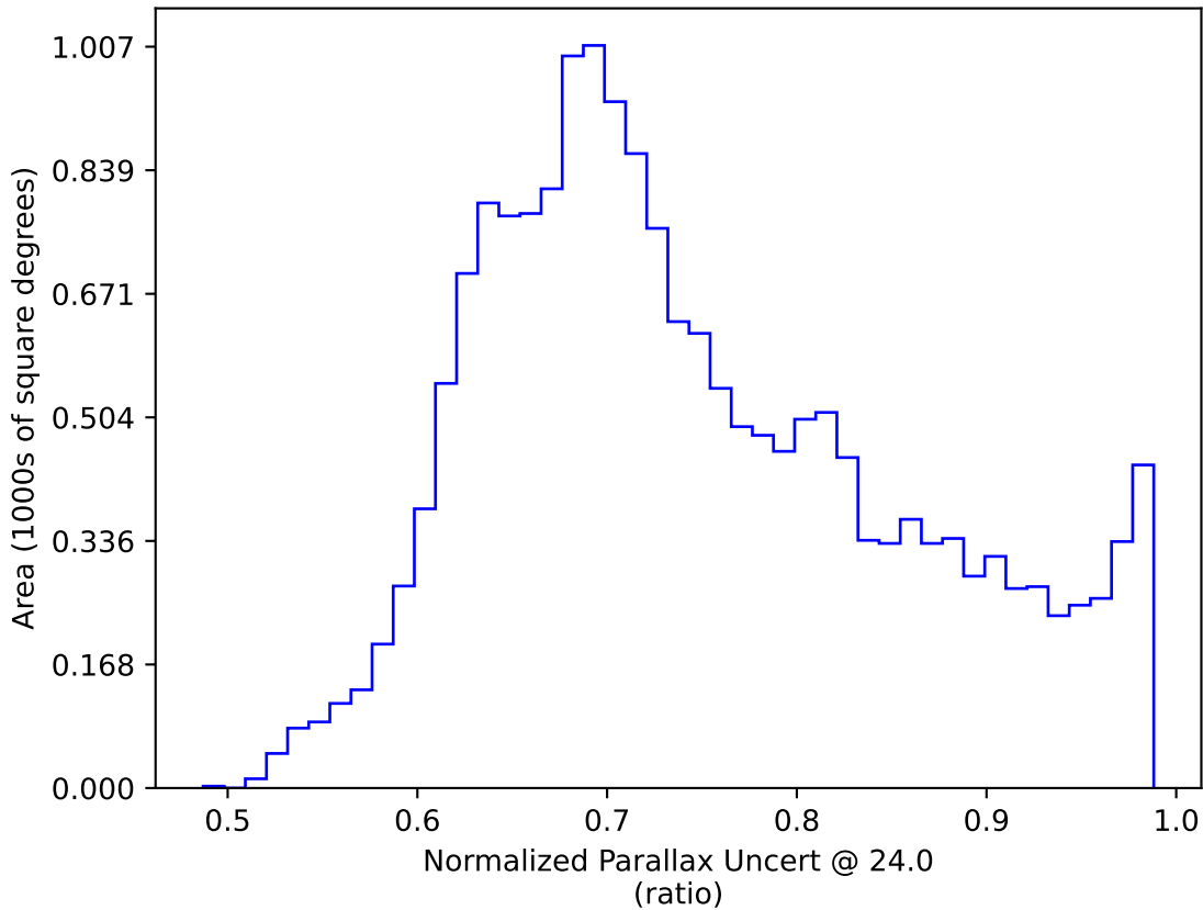
weather_cloudso10v3.4_10yrs WFD: Normalized Parallax Uncert @ 24.0
