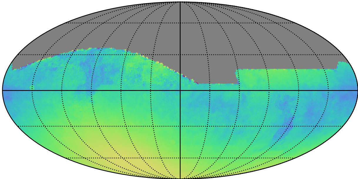
weather_cloudso10v3.4_10yrs All sky: Normalized Parallax Uncert @ 24.0
