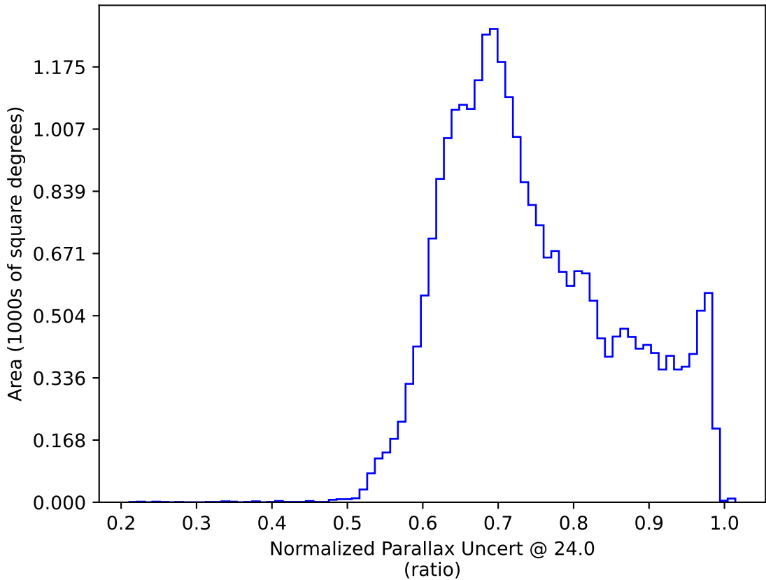
weather_cloudso10v3.4_10yrs All sky: Normalized Parallax Uncert @ 24.0
