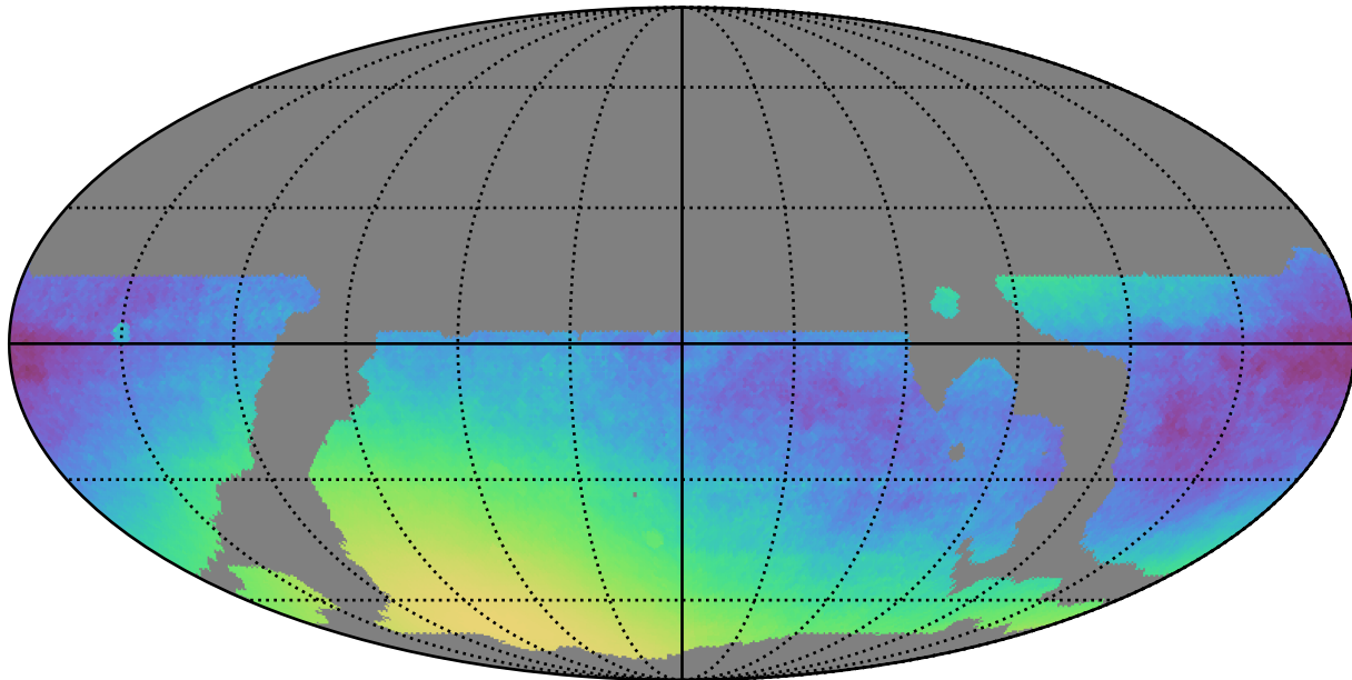
weather_cloudso10v3.4_10yrs WFD: Normalized Parallax Uncert @ 22.4
