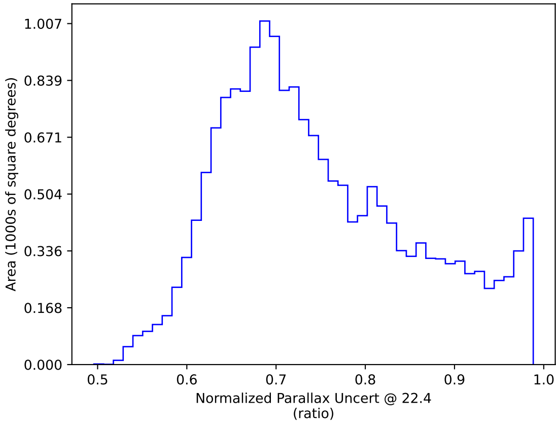
weather_cloudso10v3.4_10yrs WFD: Normalized Parallax Uncert @ 22.4
