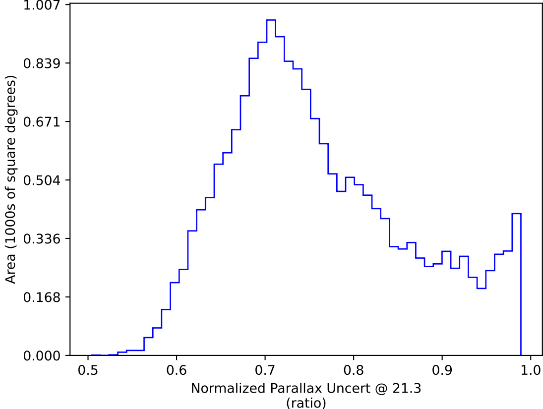
weather_cloudso10v3.4_10yrs WFD y band only: Normalized Parallax Uncert @ 21.3
