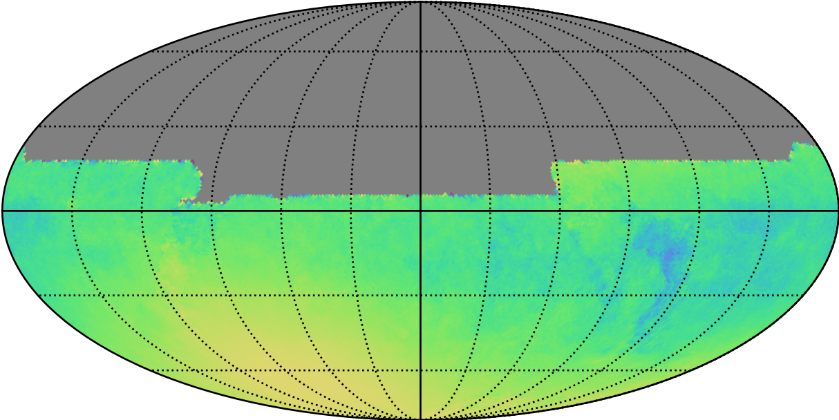
weather_cloudso10v3.4_10yrs All sky y band only: Normalized Parallax Uncert @ 21.3
