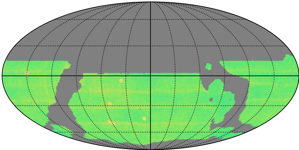
weather_cloudso10v3.4_10yrs WFD all bands: N Unique Nights
