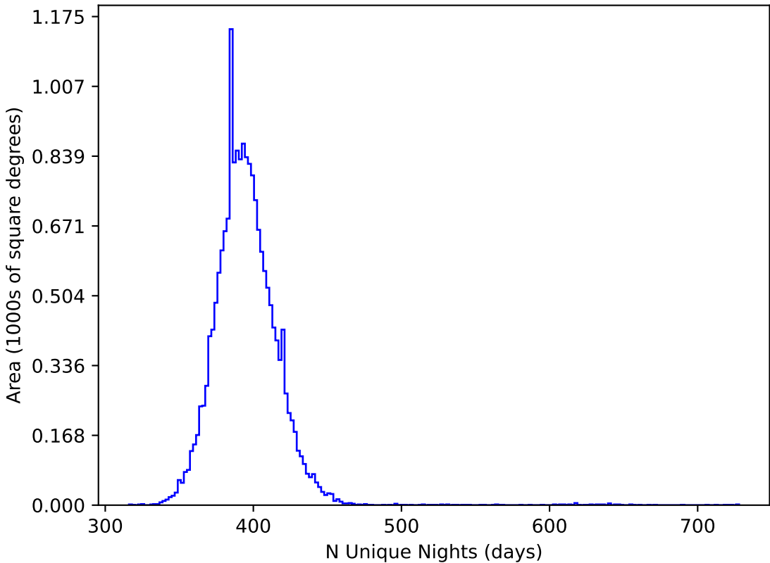
weather_cloudso10v3.4_10yrs WFD all bands: N Unique Nights
