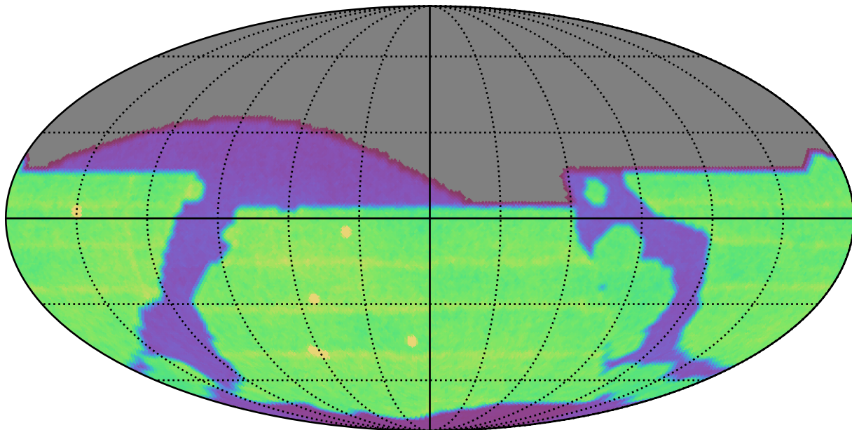
weather_cloudso10v3.4_10yrs All sky all bands: N Unique Nights
