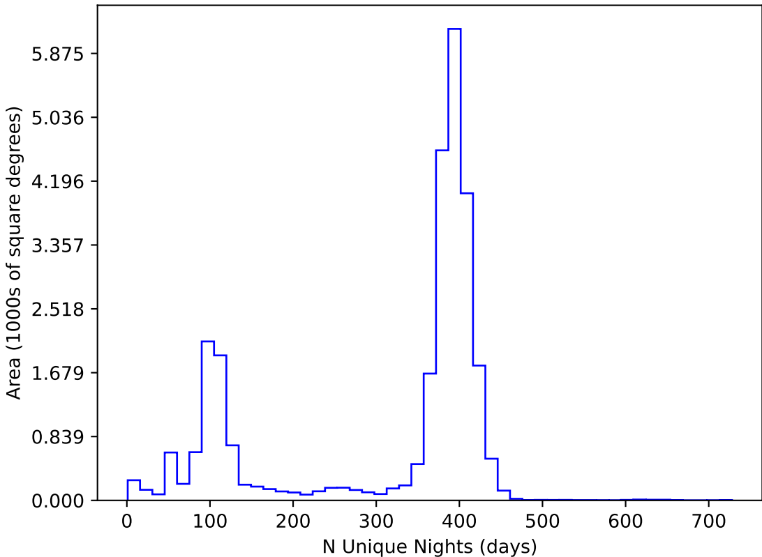
weather_cloudso10v3.4_10yrs All sky all bands: N Unique Nights
