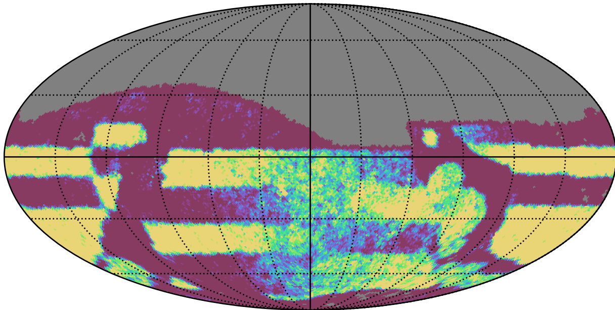
weather_cloudso10v3.4_10yrs Yr 3-4 r band: NVisits
