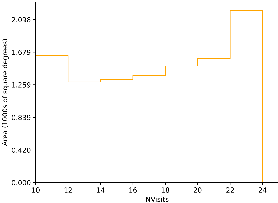
weather_cloudso10v3.4_10yrs Yr 3-4 r band: NVisits
