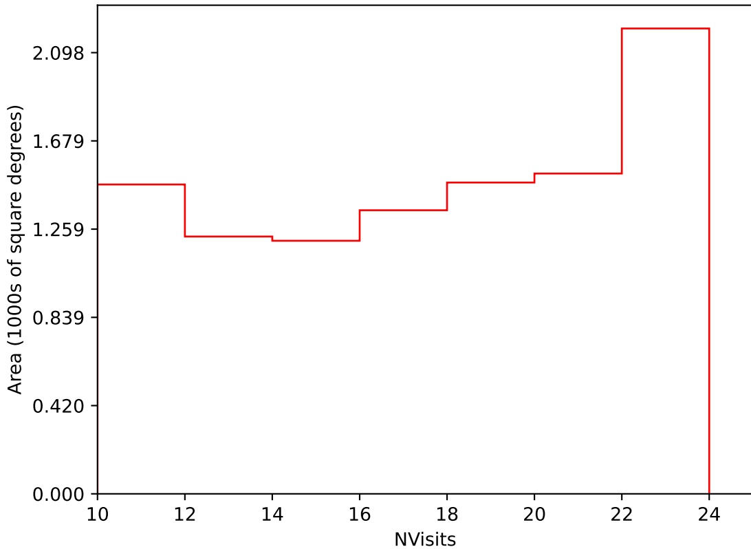
weather_cloudso10v3.4_10yrs Yr 3-4 i band: NVisits
