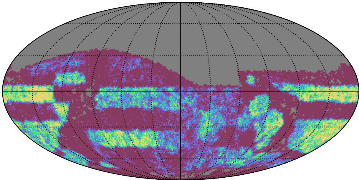
weather_cloudso10v3.4_10yrs Yr 3-4 g band: NVisits
