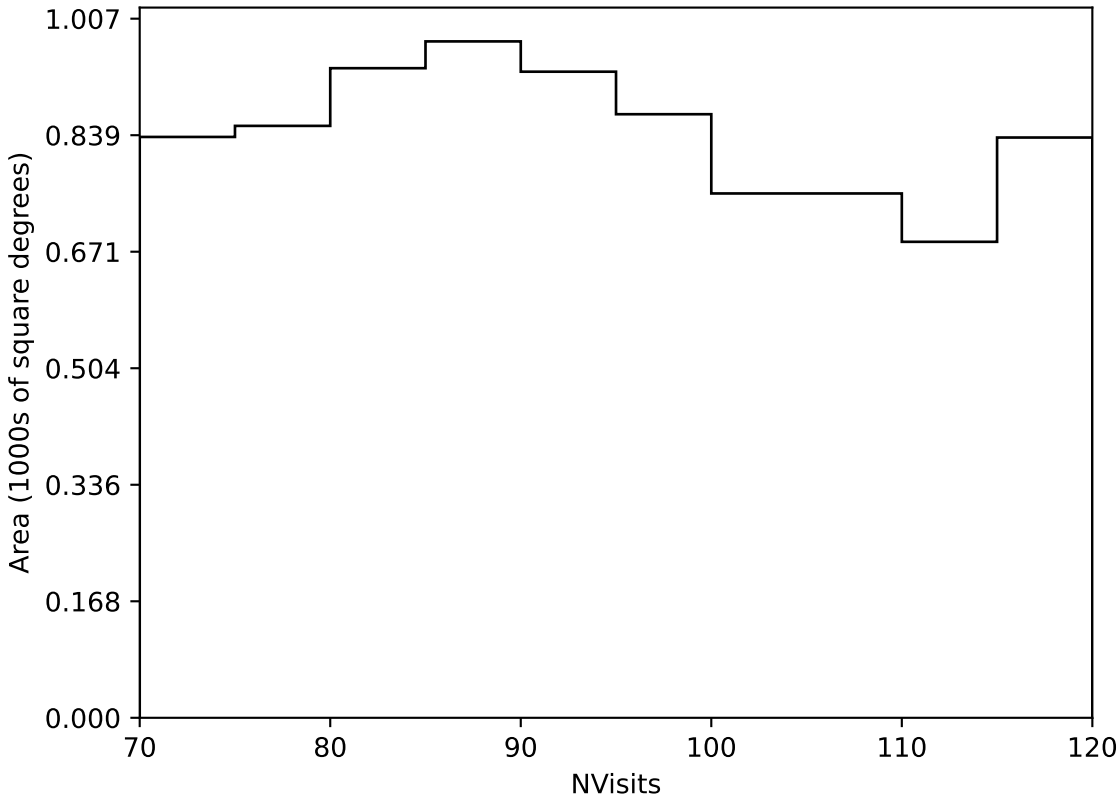
weather_cloudso10v3.4_10yrs Yr 3-4 all bands: NVisits
