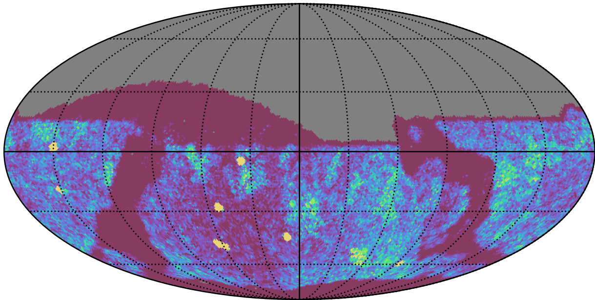
weather_cloudso10v3.4_10yrs Yr 1 z band: NVisits
