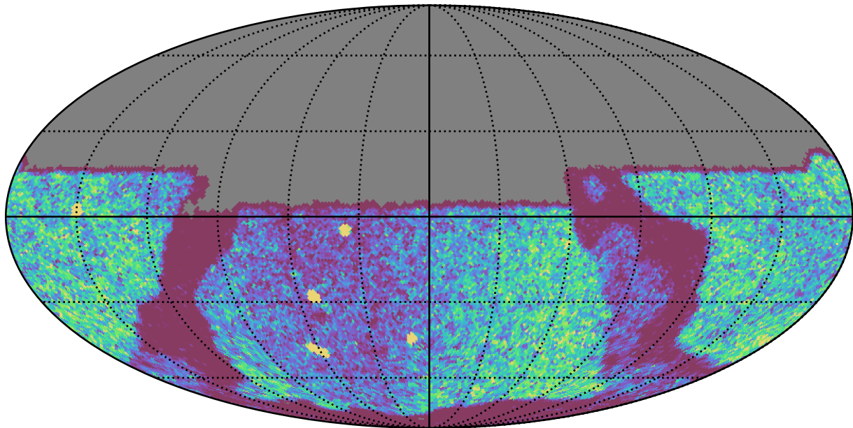
weather_cloudso10v3.4_10yrs Yr 1 y band: NVisits
