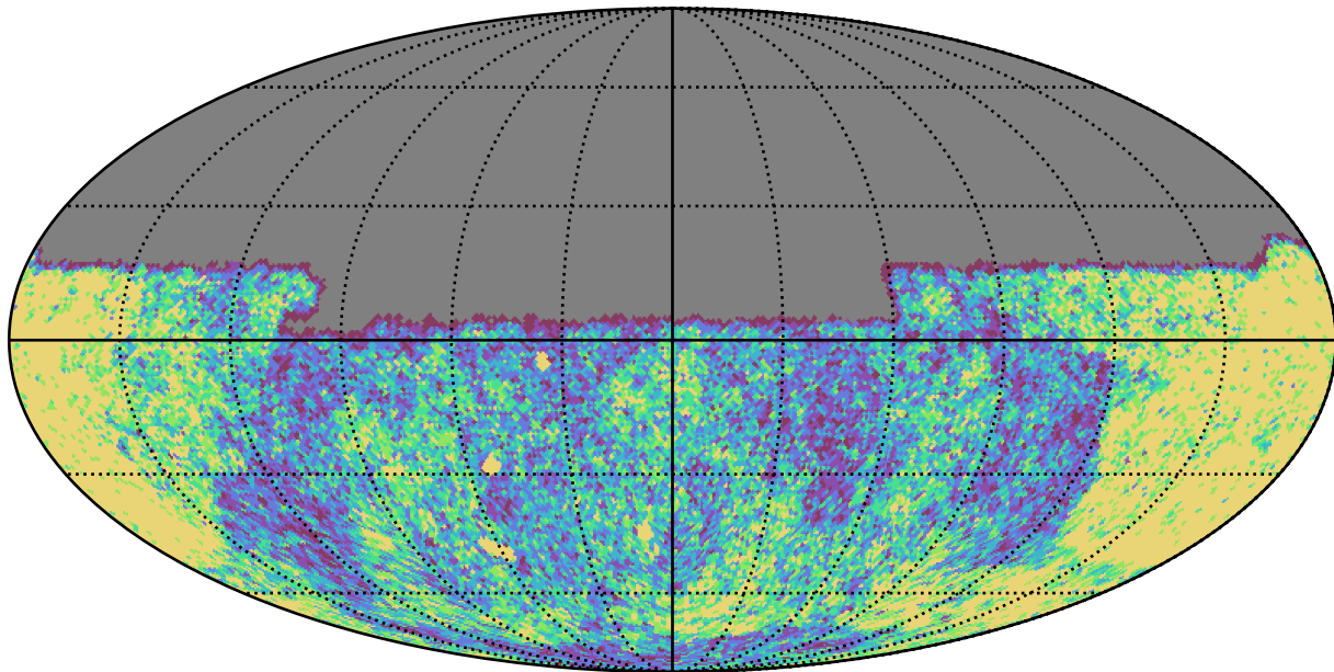
weather_cloudso10v3.4_10yrs Yr 1 u band: NVisits
