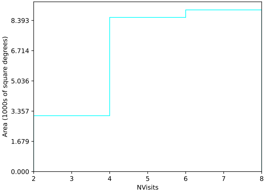
weather_cloudso10v3.4_10yrs Yr 1 u band: NVisits
