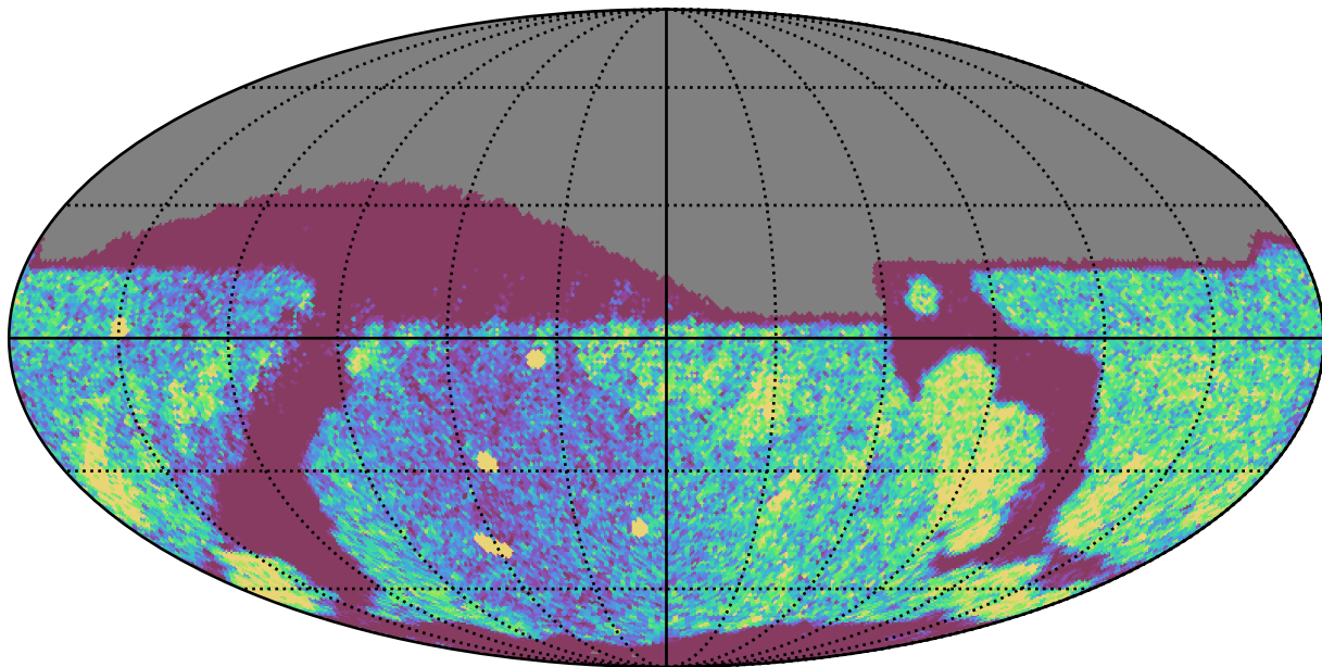
weather_cloudso10v3.4_10yrs Yr 1 r band: NVisits
