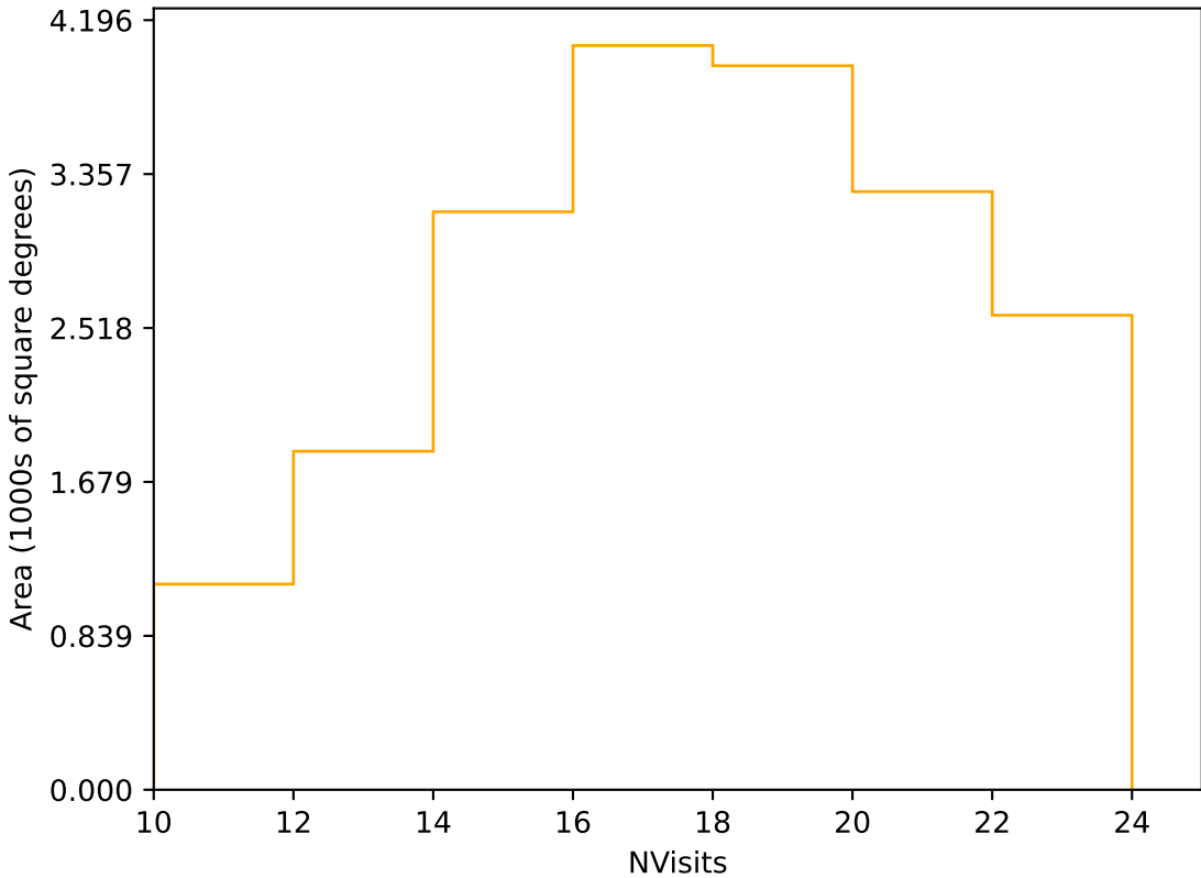
weather_cloudso10v3.4_10yrs Yr 1 r band: NVisits
