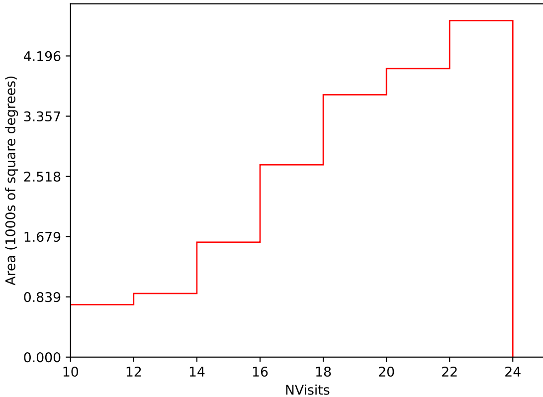
weather_cloudso10v3.4_10yrs Yr 1 i band: NVisits
