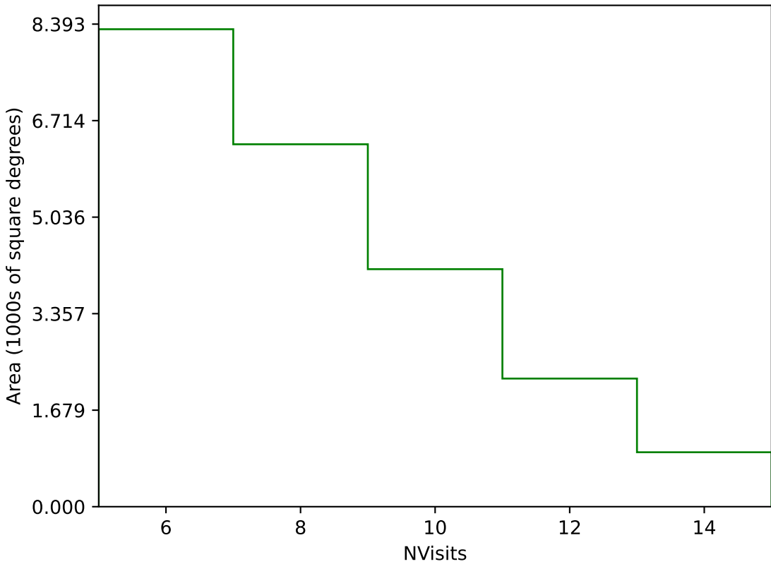
weather_cloudso10v3.4_10yrs Yr 1 g band: NVisits
