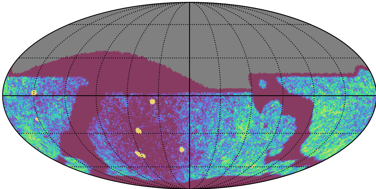
weather_cloudso10v3.4_10yrs Yr 1 all bands: NVisits
