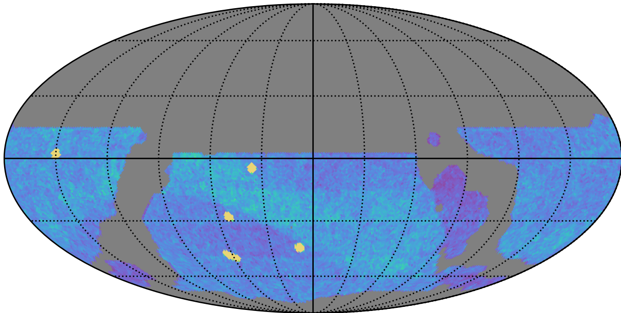
weather_cloudso10v3.4_10yrs WFD z band: NVisits
