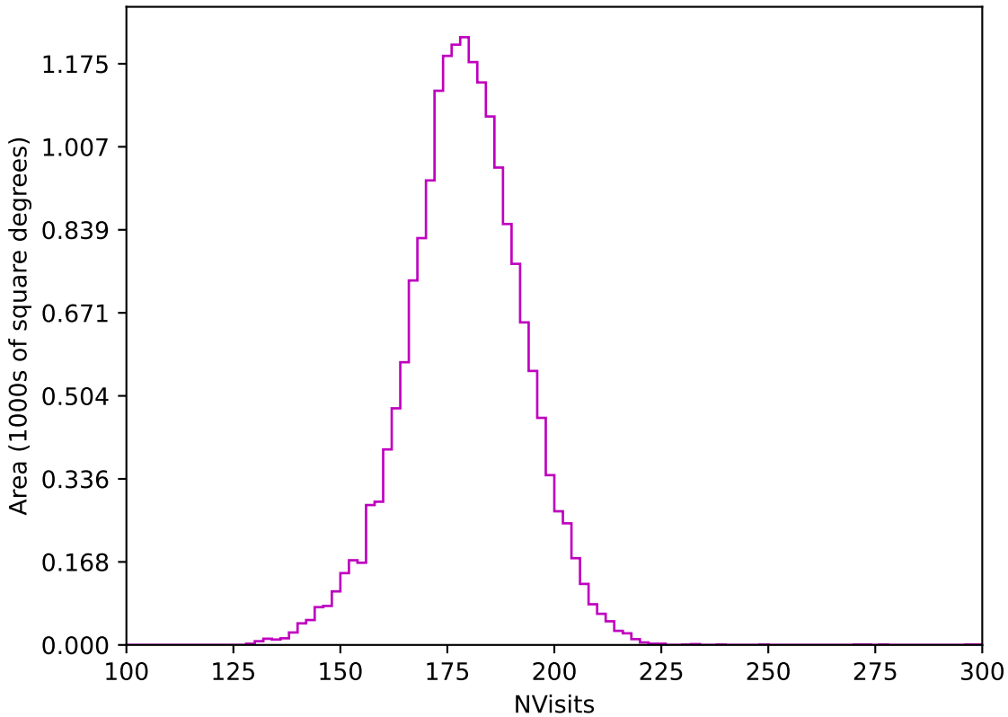
weather_cloudso10v3.4_10yrs WFD z band: NVisits
