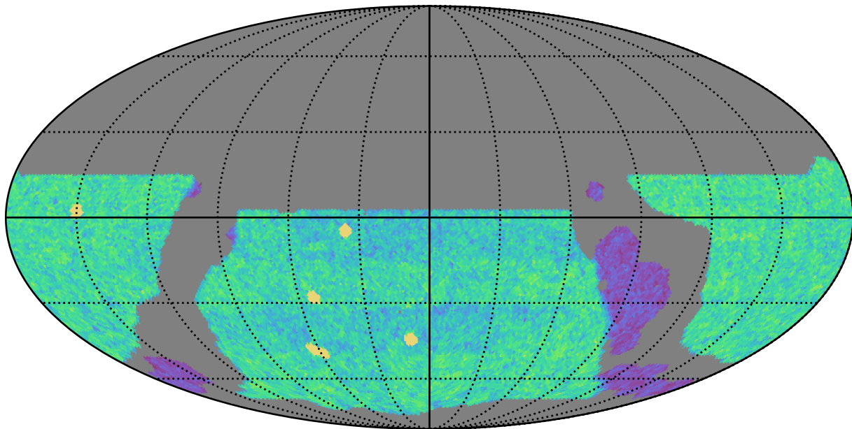
weather_cloudso10v3.4_10yrs WFD u band: NVisits
